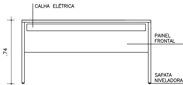
VISTA FRONTAL
