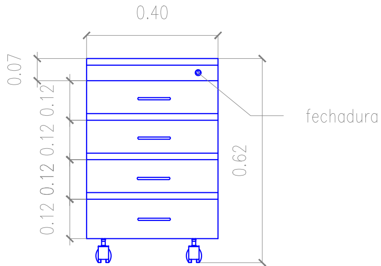
Vista Frontal
