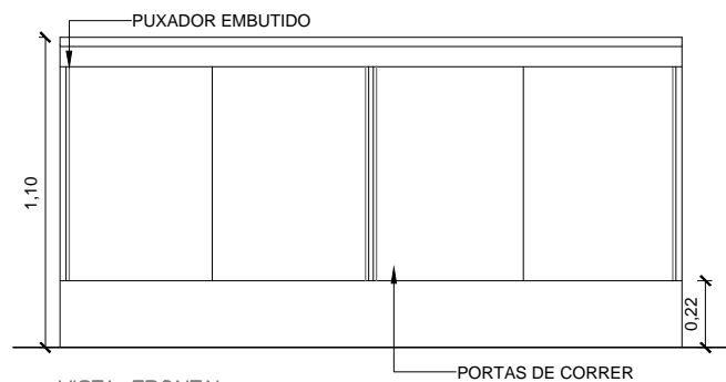
VISTA FRONTAL
